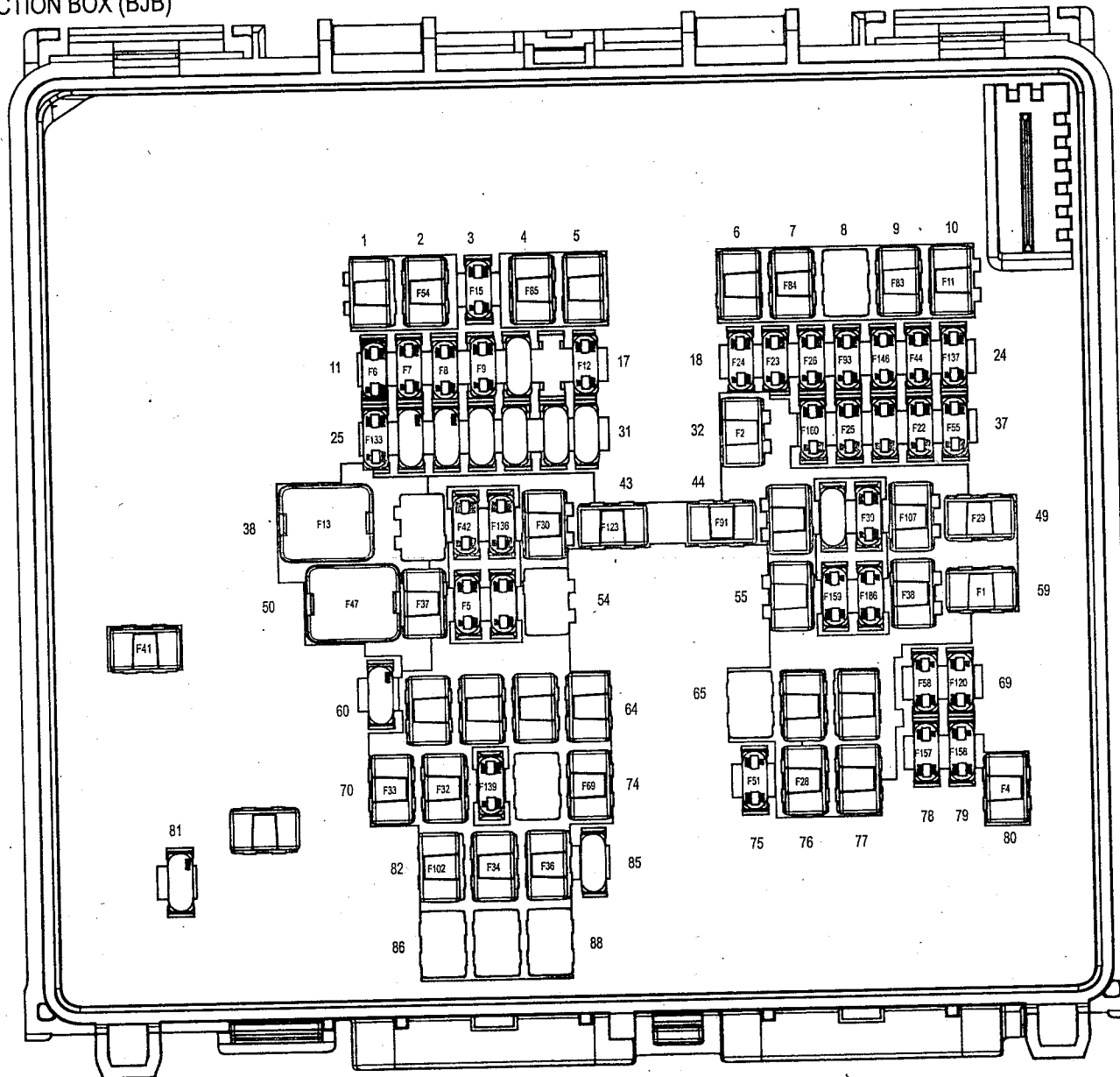
BATTERY JUNCTION BOX (BJB)
