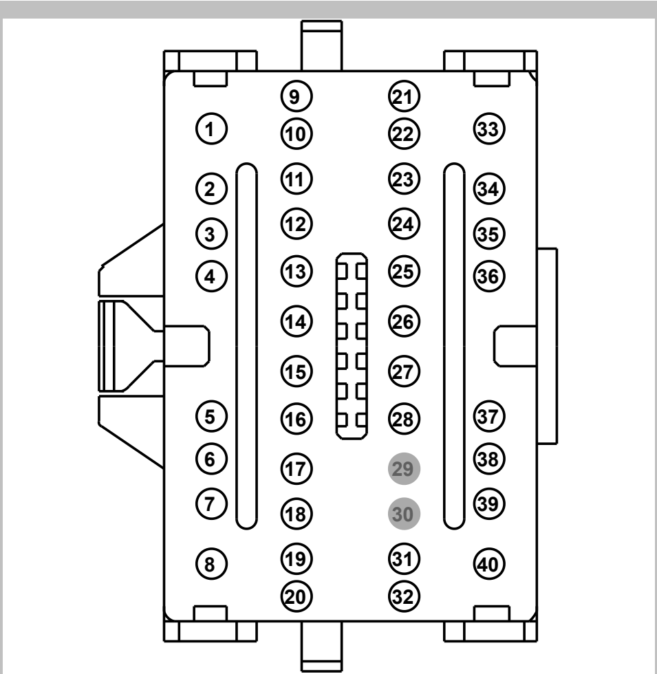
FEMALE Harness 14401
