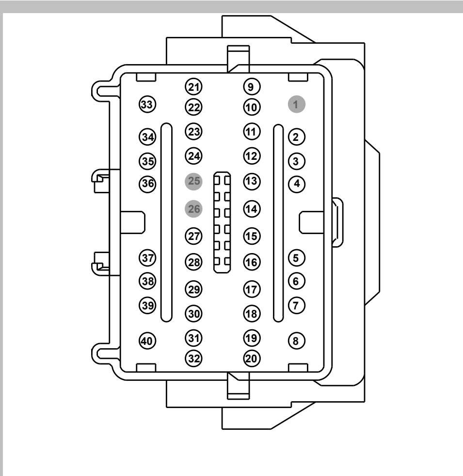
MALE Harness 14A005
